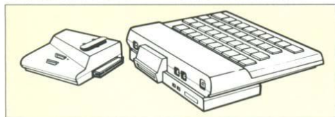
ZX Interface 2 works independently of other peripherals, plugs into rear of ZX Interface 1.
